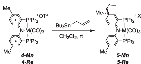
Scheme 3. Allylation of [(PNP)M(CO) 3 ]OTf
